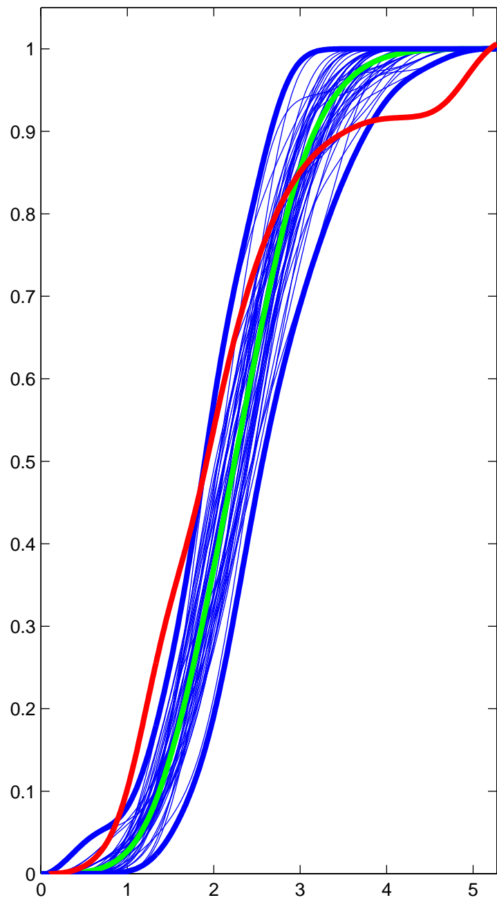
Dist to origin of data and Gauss
