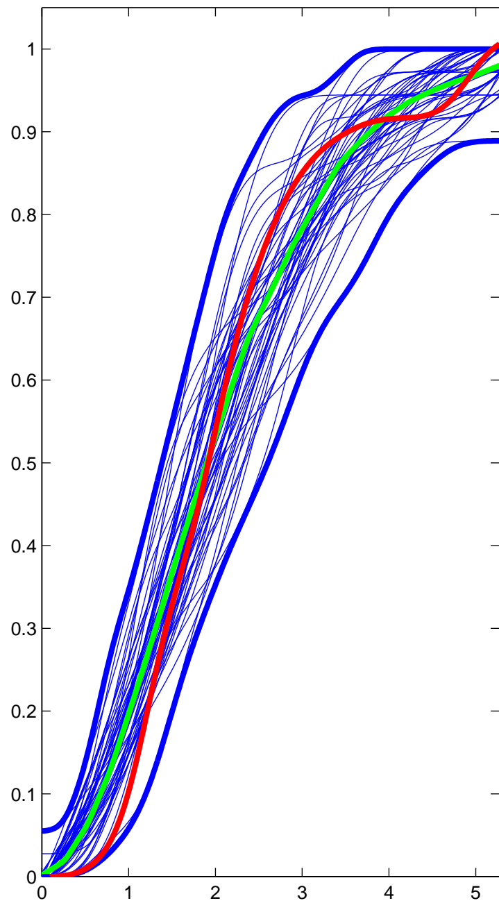
Dist to origin of data and transfd Gauss
