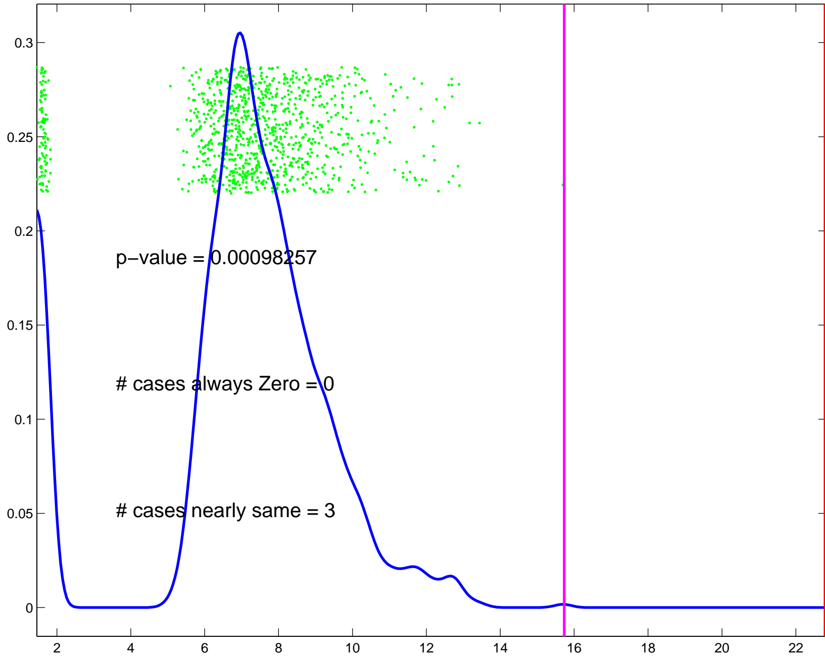
Kurtosis , IC1 Gauss. test of power transf data, max of r = 10 rep's
