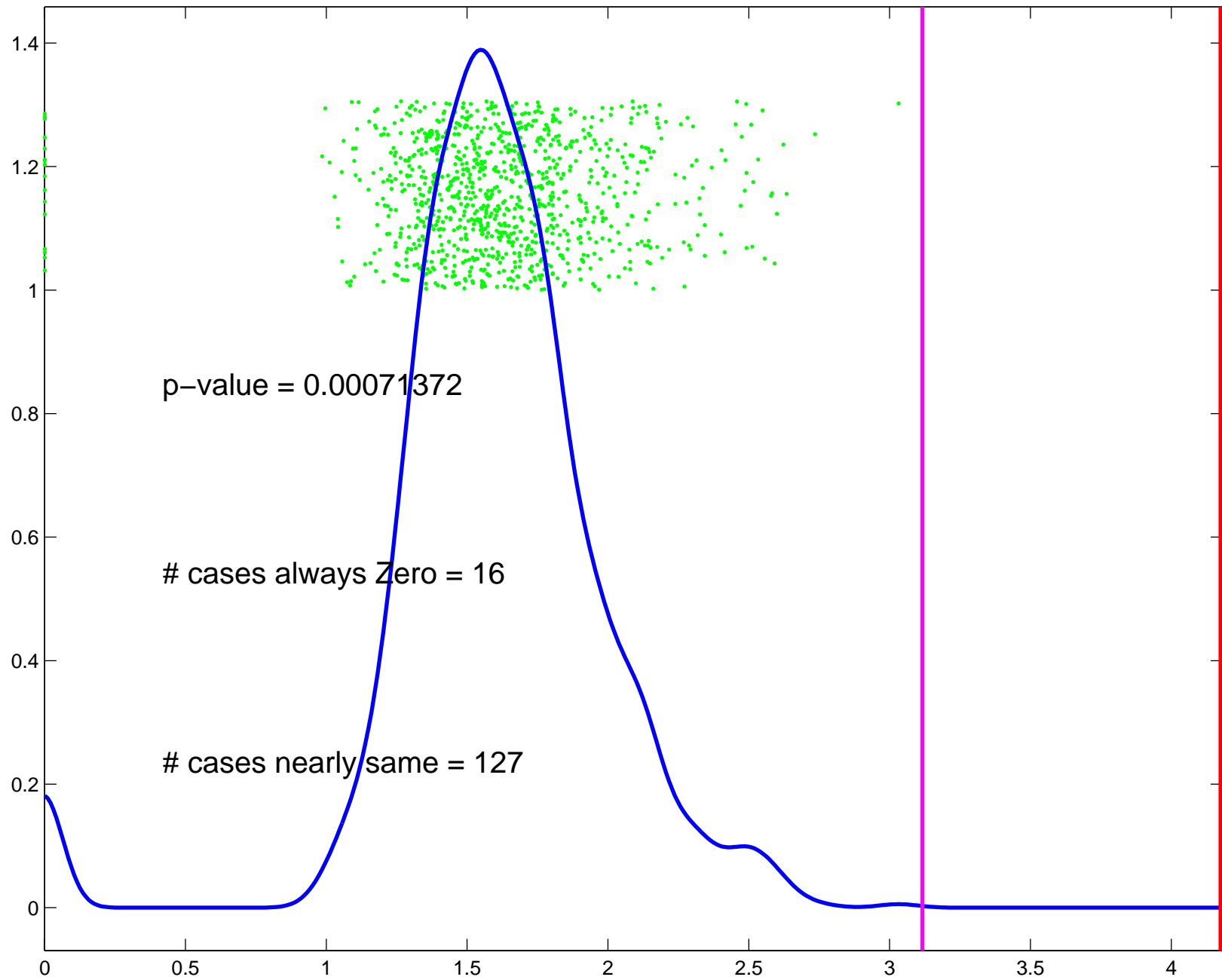
Abs Skew , IC1 Gauss. test of power transf data, max of r = 10 rep's
