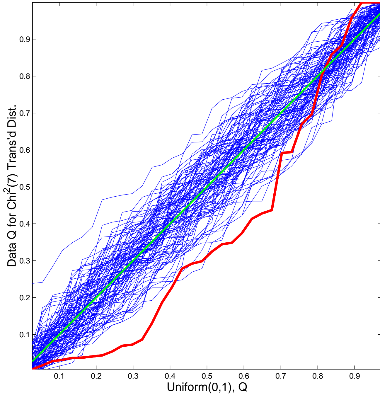
Unif. QQ for Trans'd Dist. to 0 for Sphered data
