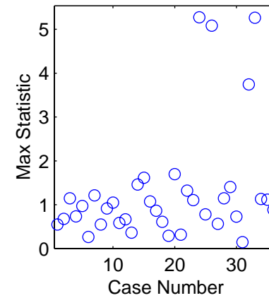
Max abs data by case, r = 1000
