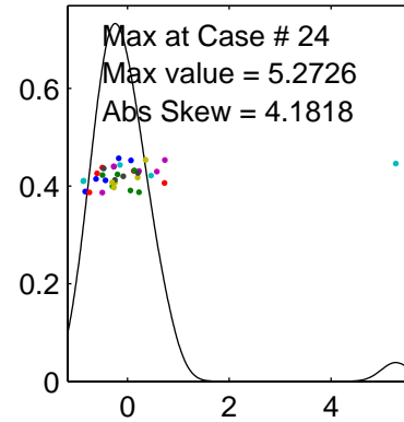
Case # of Max'r over r = 1000
