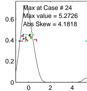
Max abs data by case, r = 1000
