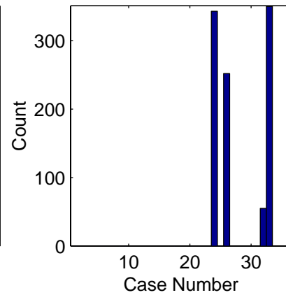
Case # of Max'r over r = 1000
