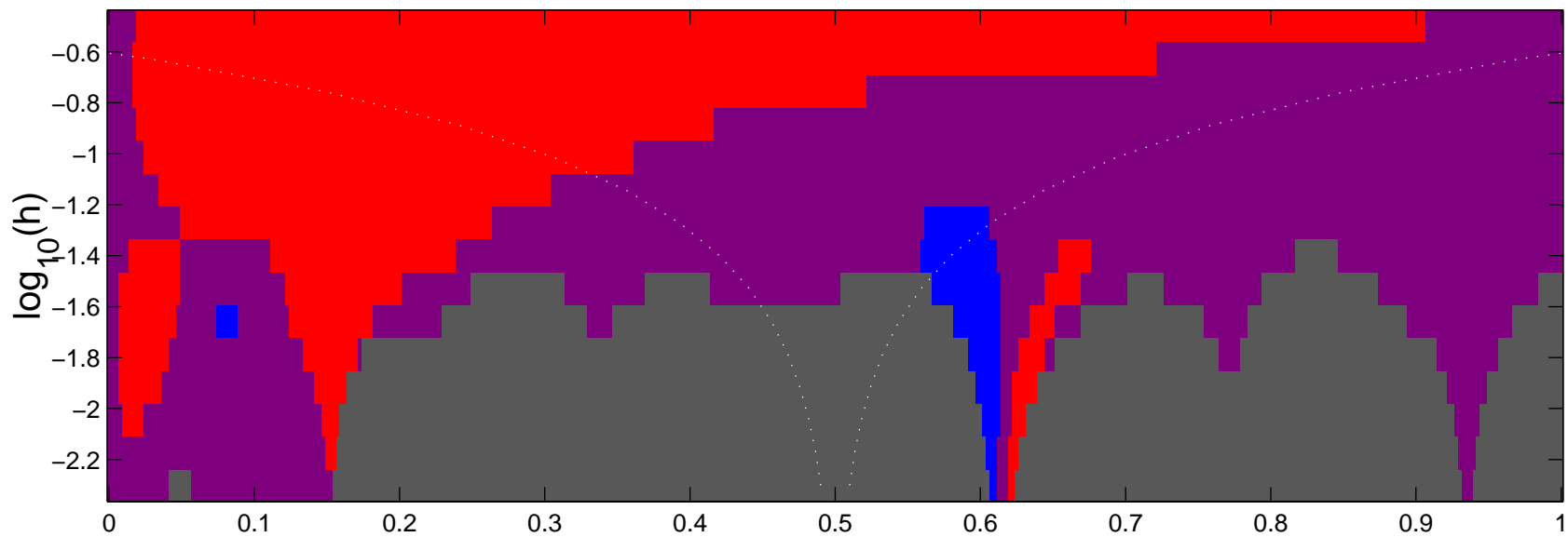
Transformed angle dist., SiZer map
