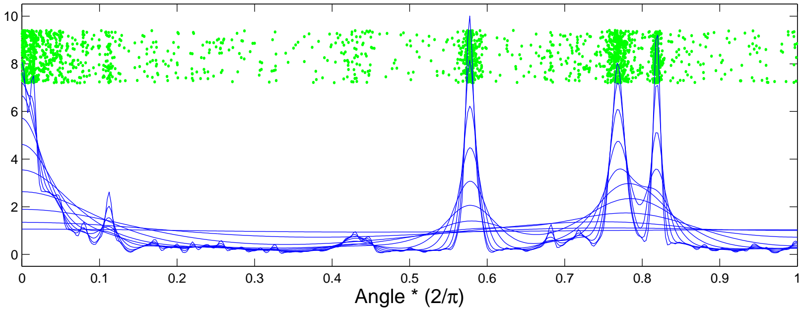
HTTP Resp. Asy. Indep. Angles, Time vs. Size, top 2000
