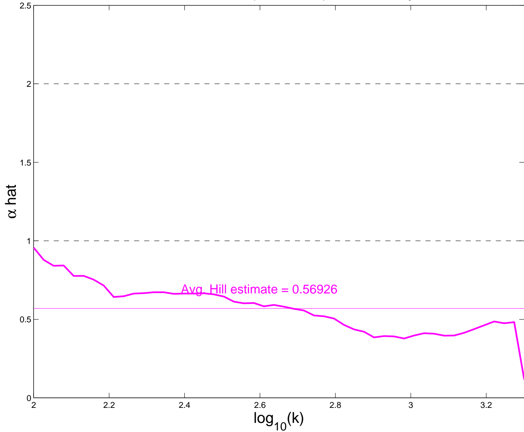
Hill estimates, HTTP Ratio (Size/Time), Wednesday, Afternoon
