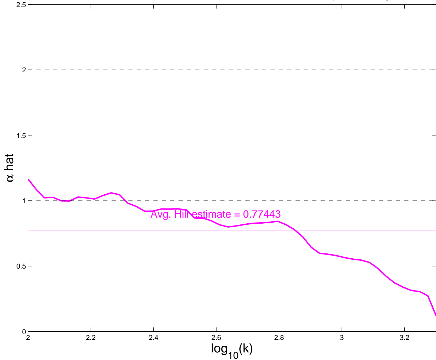
Hill estimates, HTTP Ratio (Size/Time), Sunday, Evening
