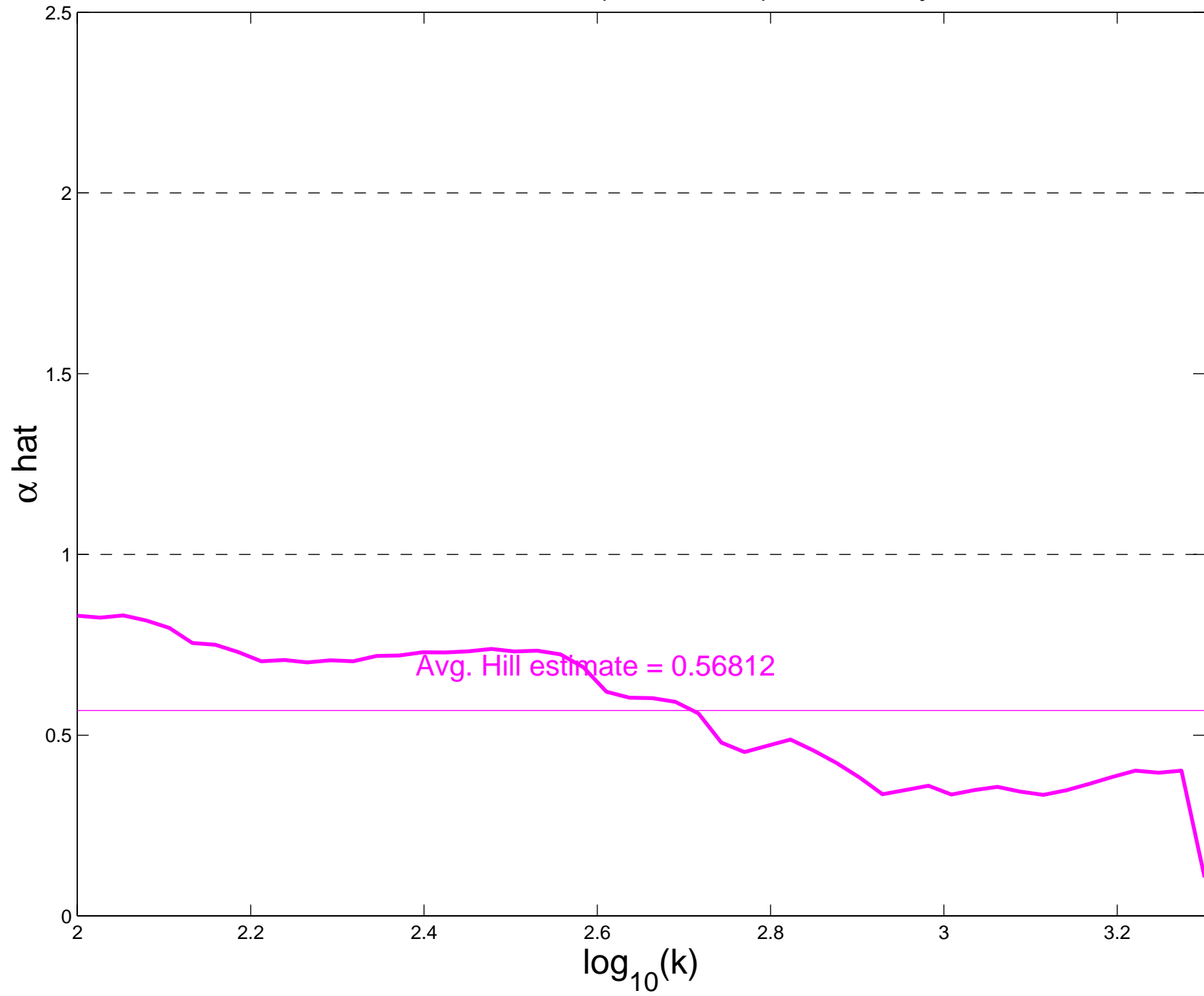
Hill estimates, HTTP Ratio (Size/Time), Thursday, Afternoon
