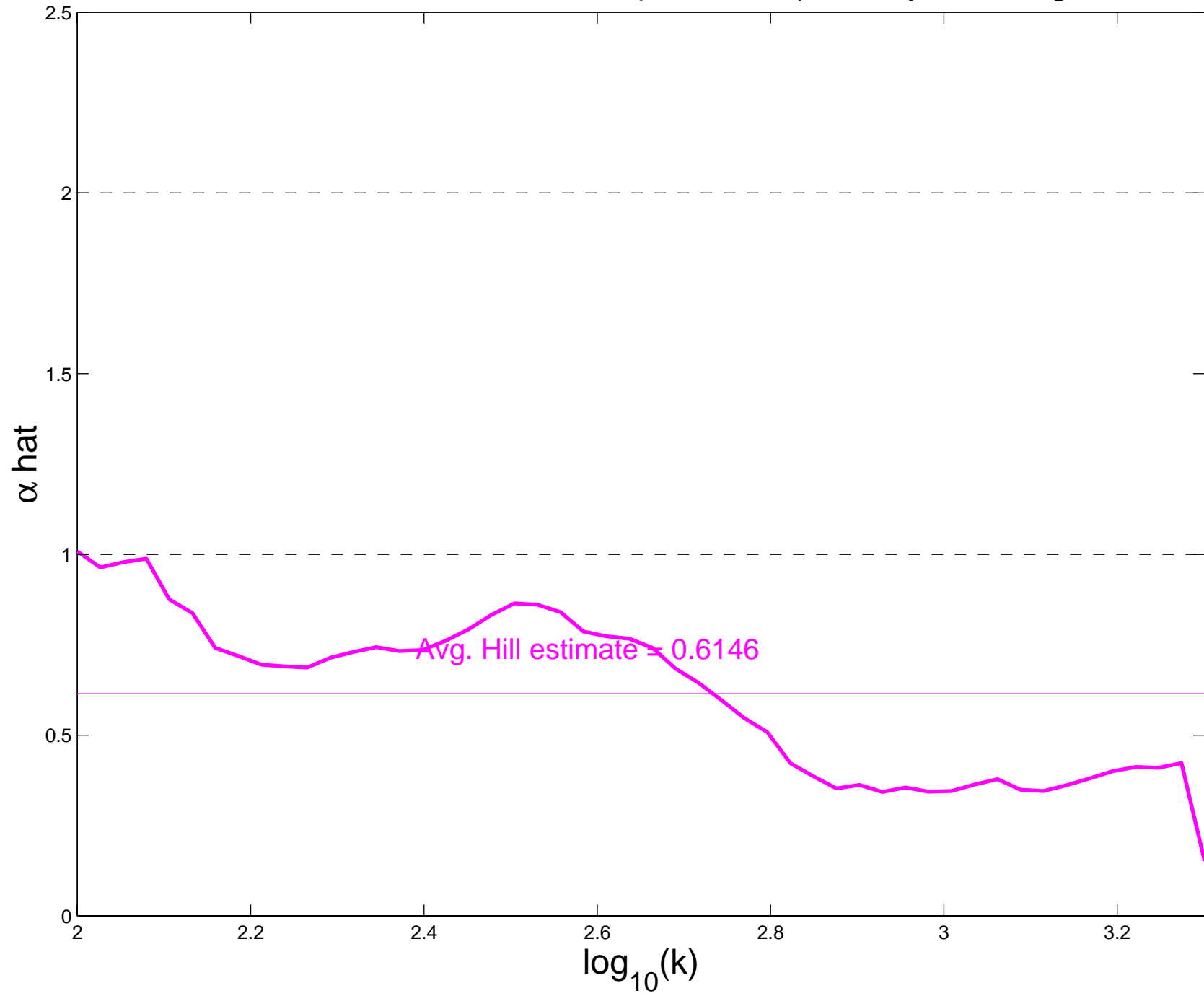
Hill estimates, HTTP Ratio (Size/Time), Friday, Morning
