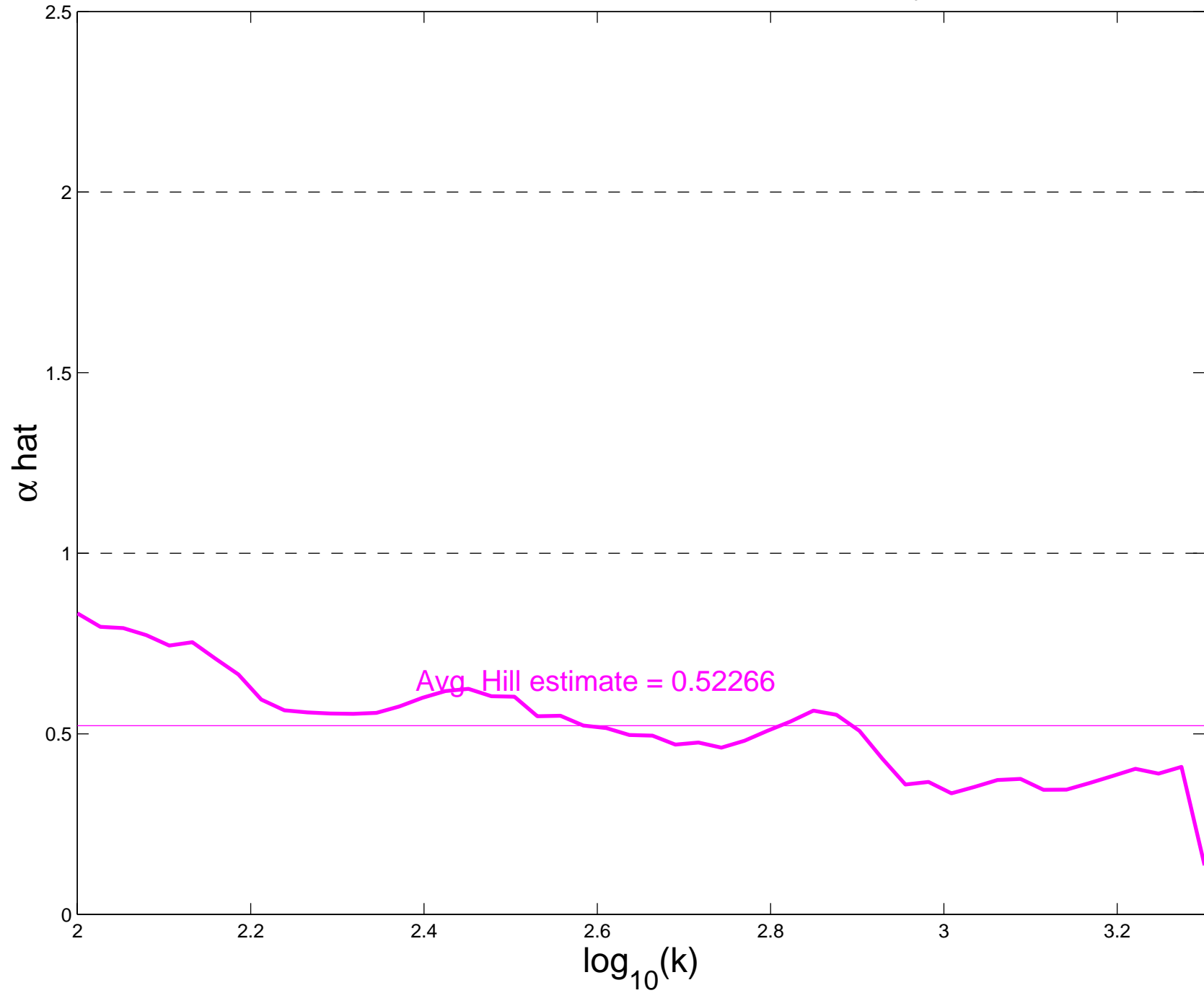
Hill estimates, HTTP Ratio (Size/Time), Tuesday, Afternoon
