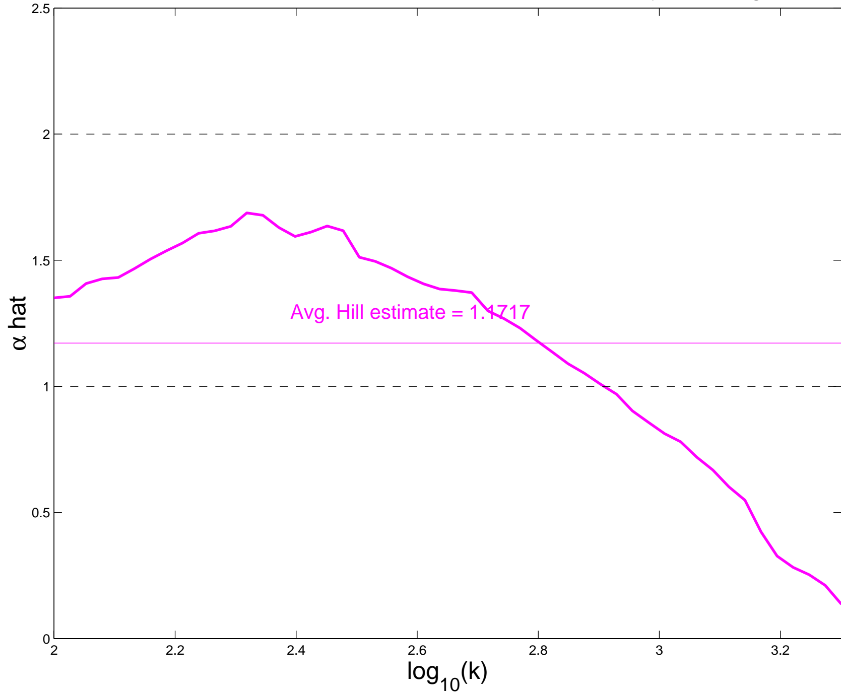
Hill estimates, HTTP Ratio (Size/Time), Thursday, Evening
