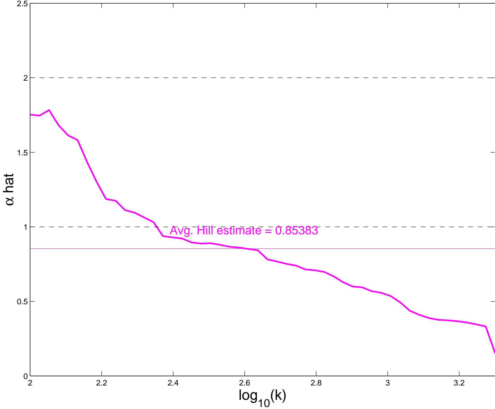
Hill estimates, HTTP Ratio (Size/Time), Saturday, Afternoon
