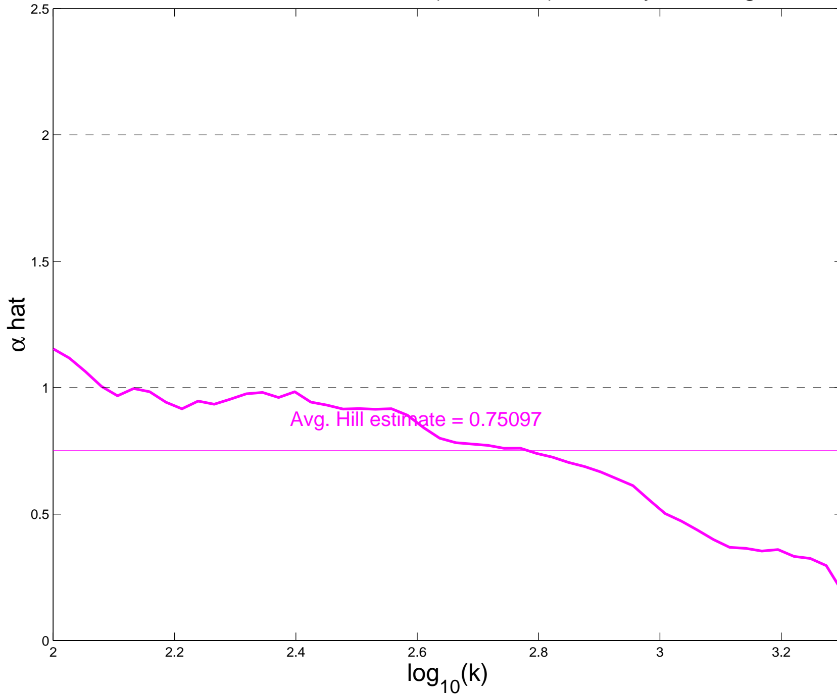
Hill estimates, HTTP Ratio (Size/Time), Monday, Evening
