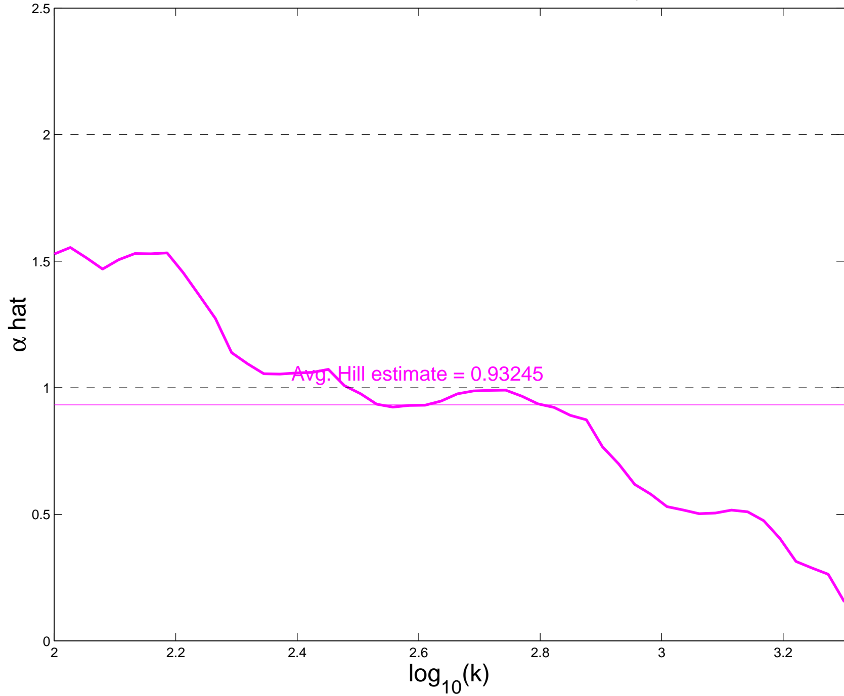
Hill estimates, HTTP Ratio (Size/Time), Sunday, Afternoon
