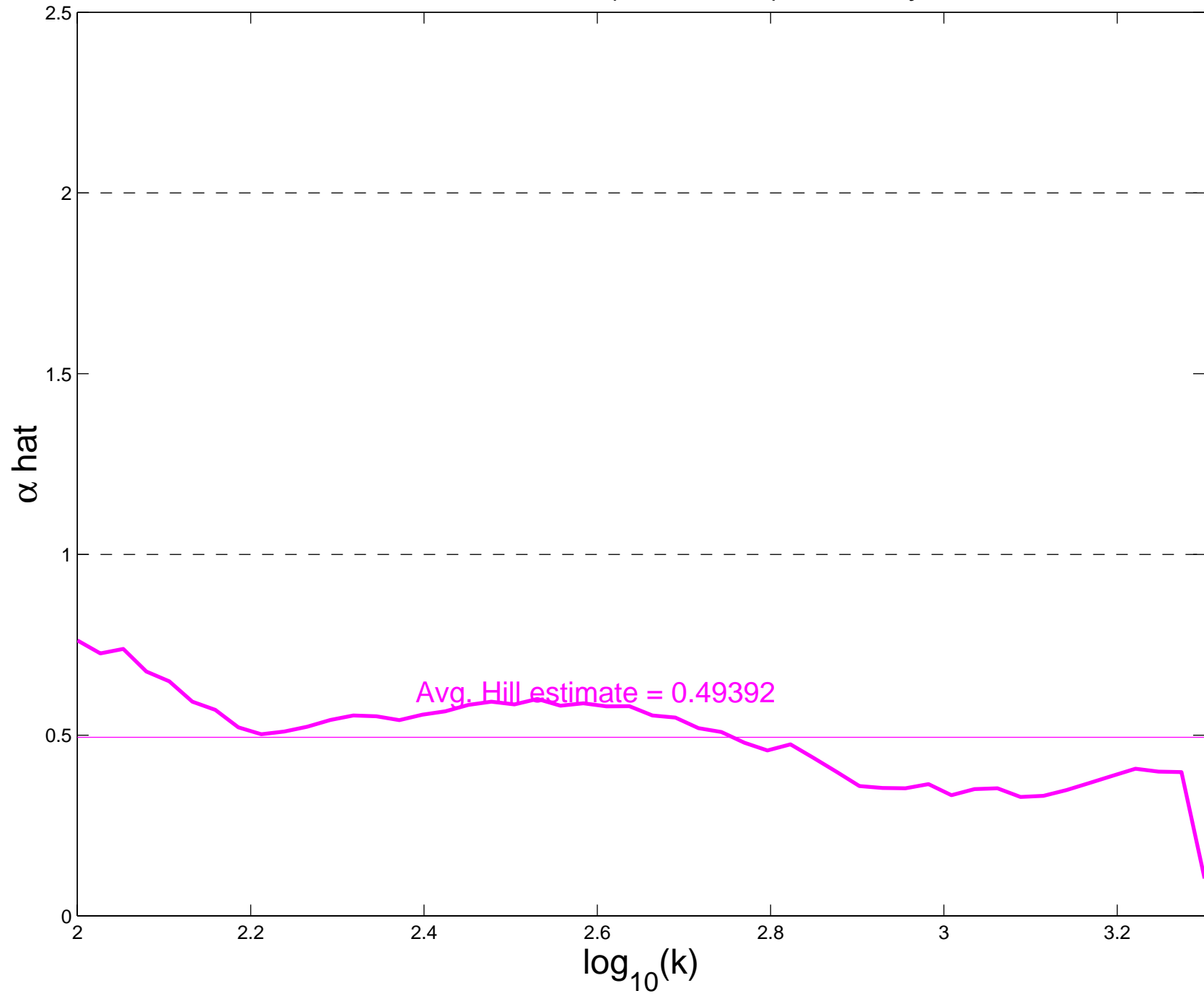
Hill estimates, HTTP Ratio (Size/Time), Monday, Afternoon
