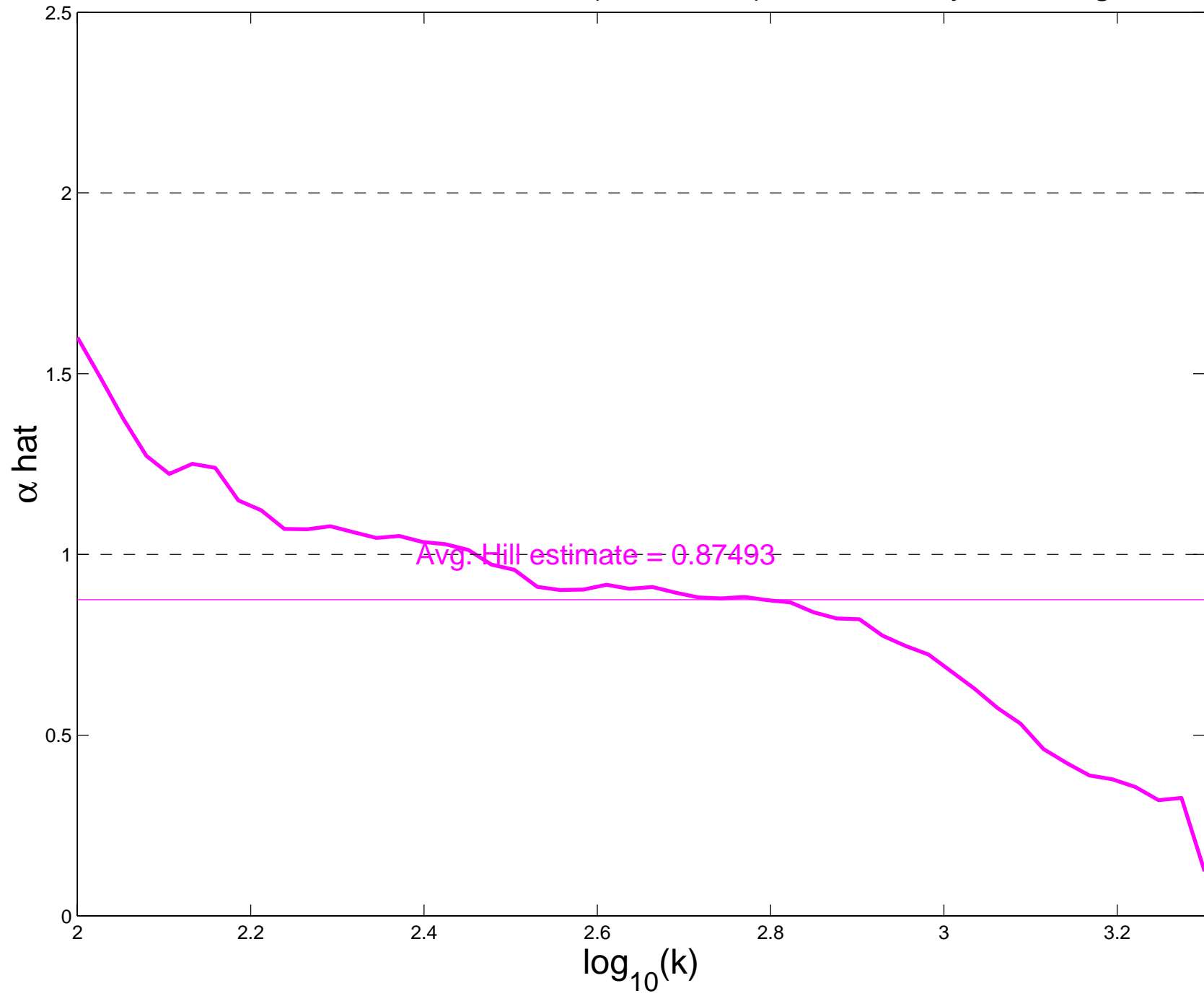
Hill estimates, HTTP Ratio (Size/Time), Wednesday, Evening
