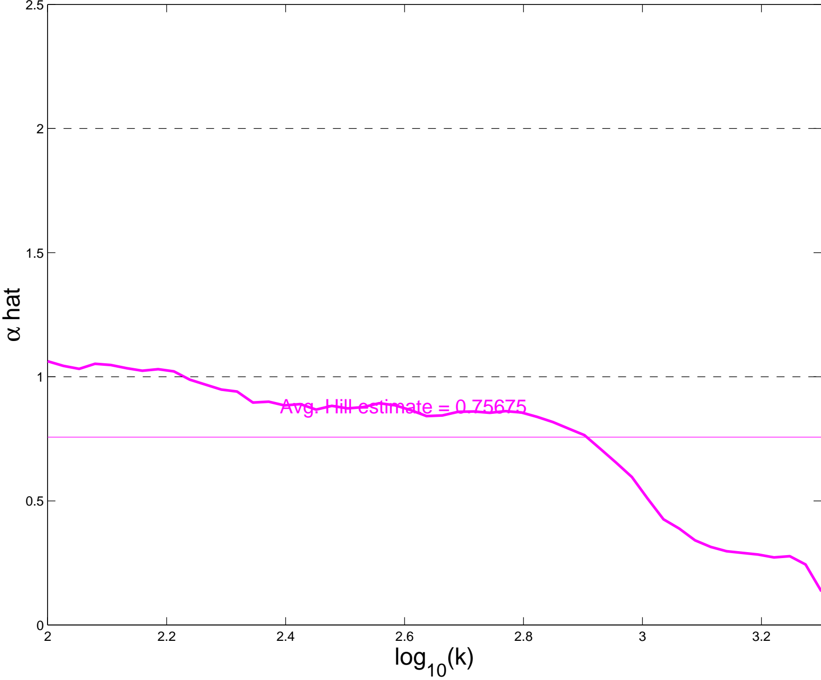
Hill estimates, HTTP Ratio (Size/Time), Tuesday, Evening
