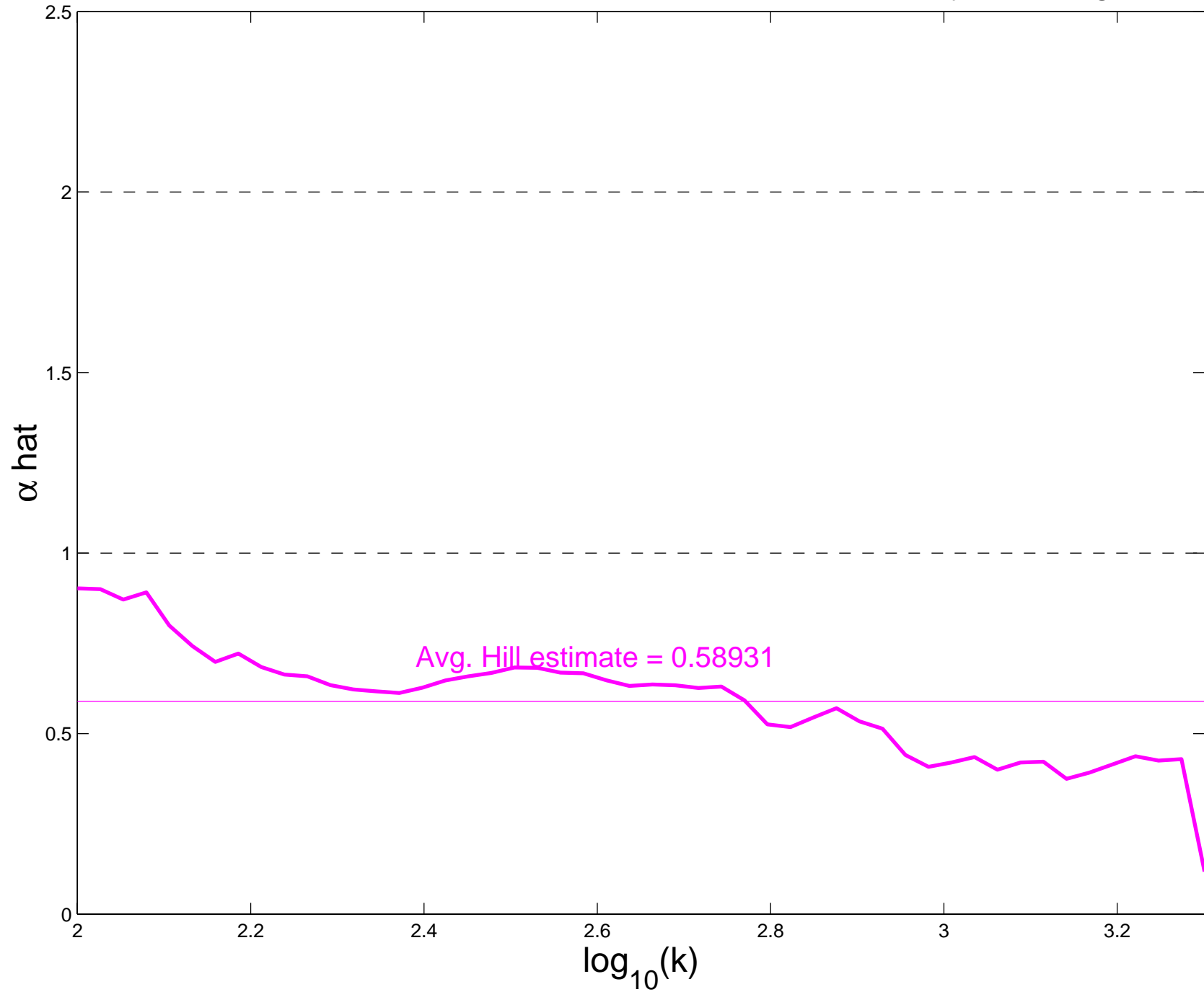
Hill estimates, HTTP Ratio (Size/Time), Wednesday, Morning
