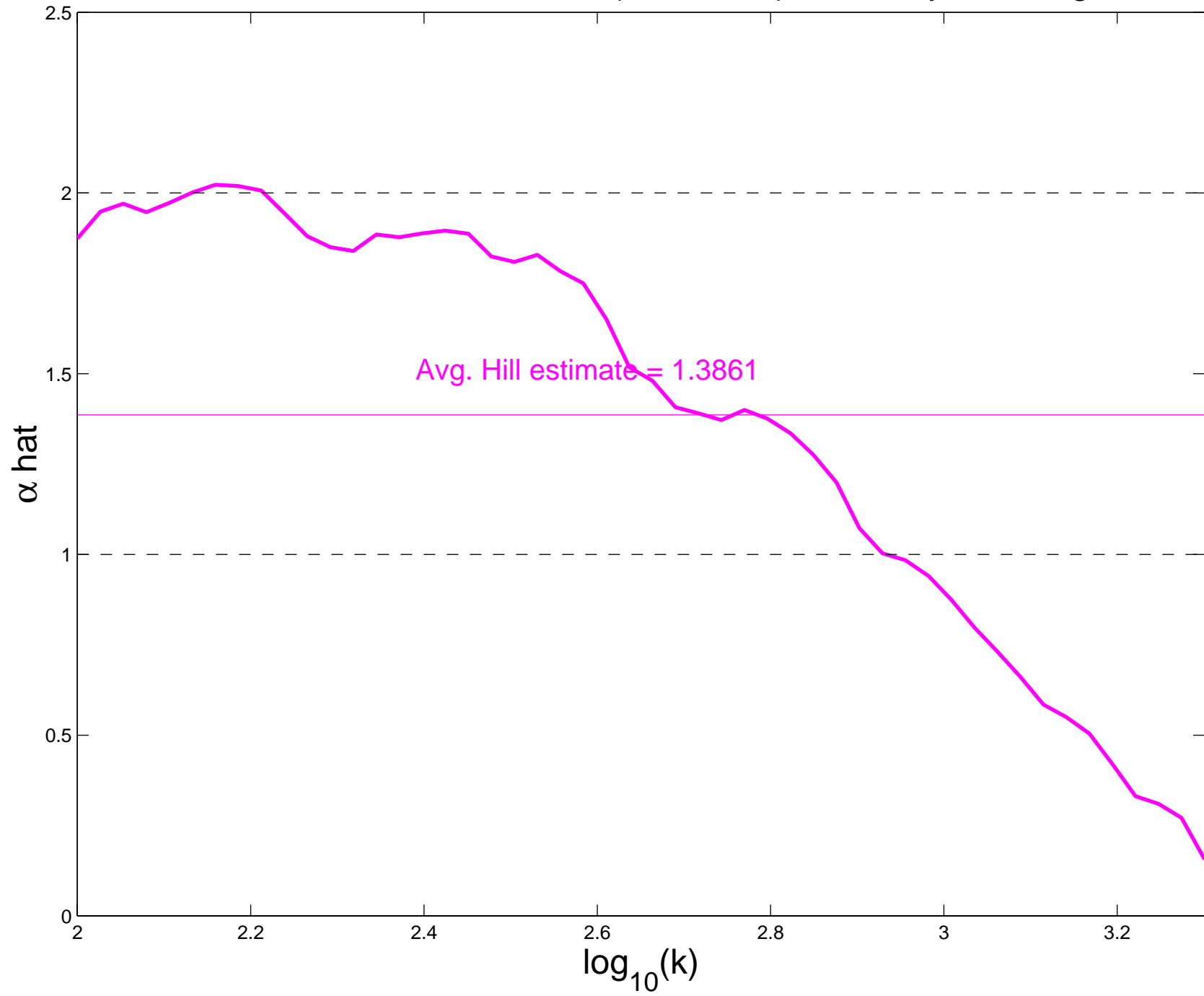
Hill estimates, HTTP Ratio (Size/Time), Saturday, Evening
