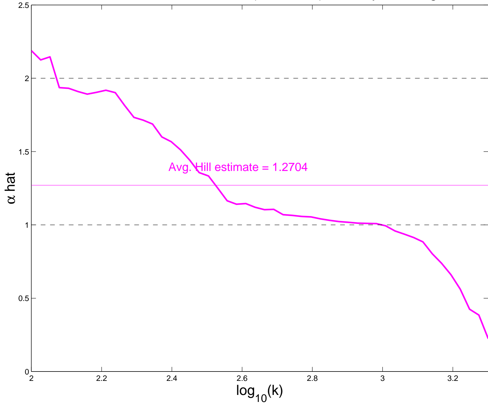
Hill estimates, HTTP Ratio (Size/Time), Sunday, Morning
