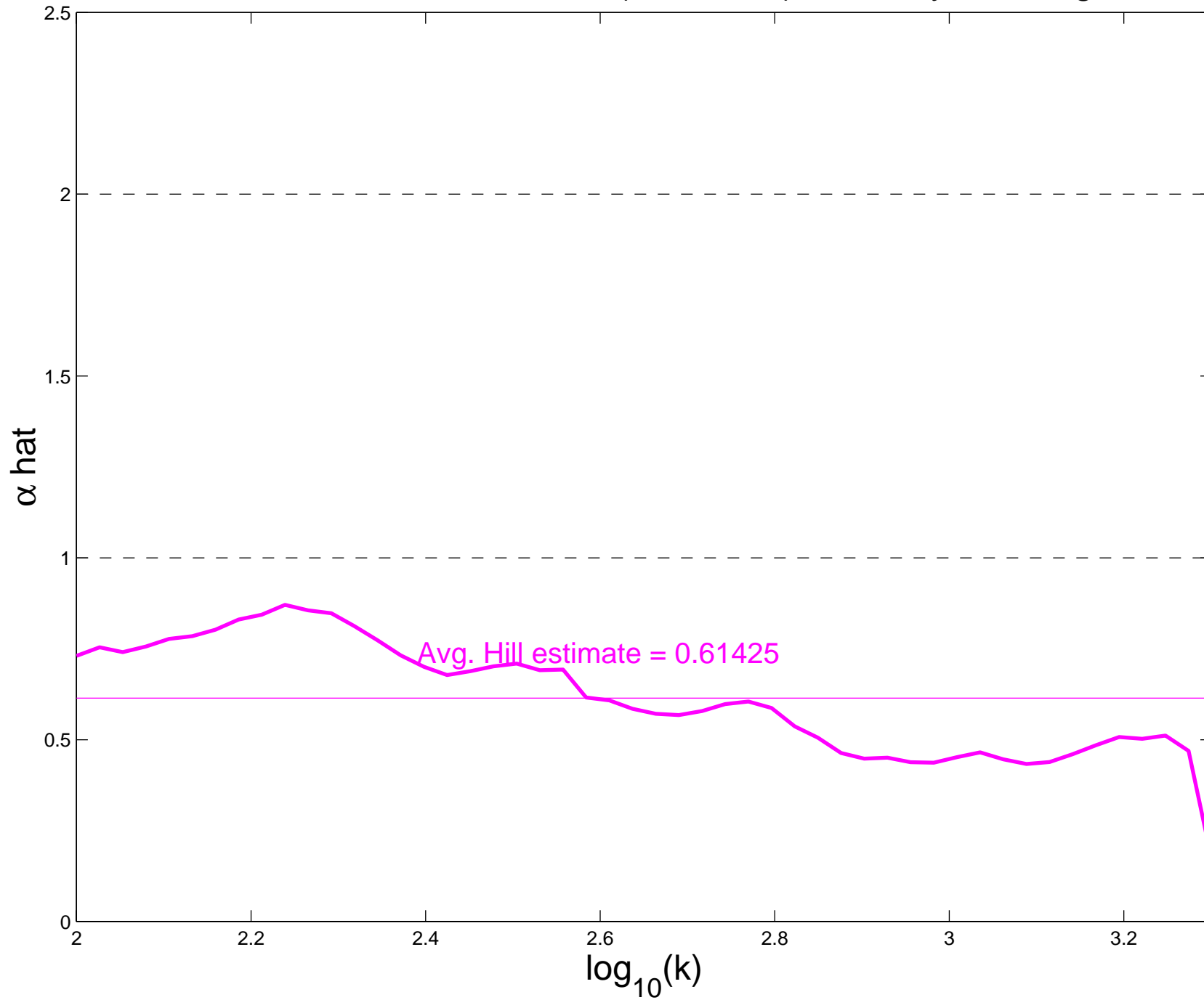
Hill estimates, HTTP Ratio (Size/Time), Tuesday, Morning
