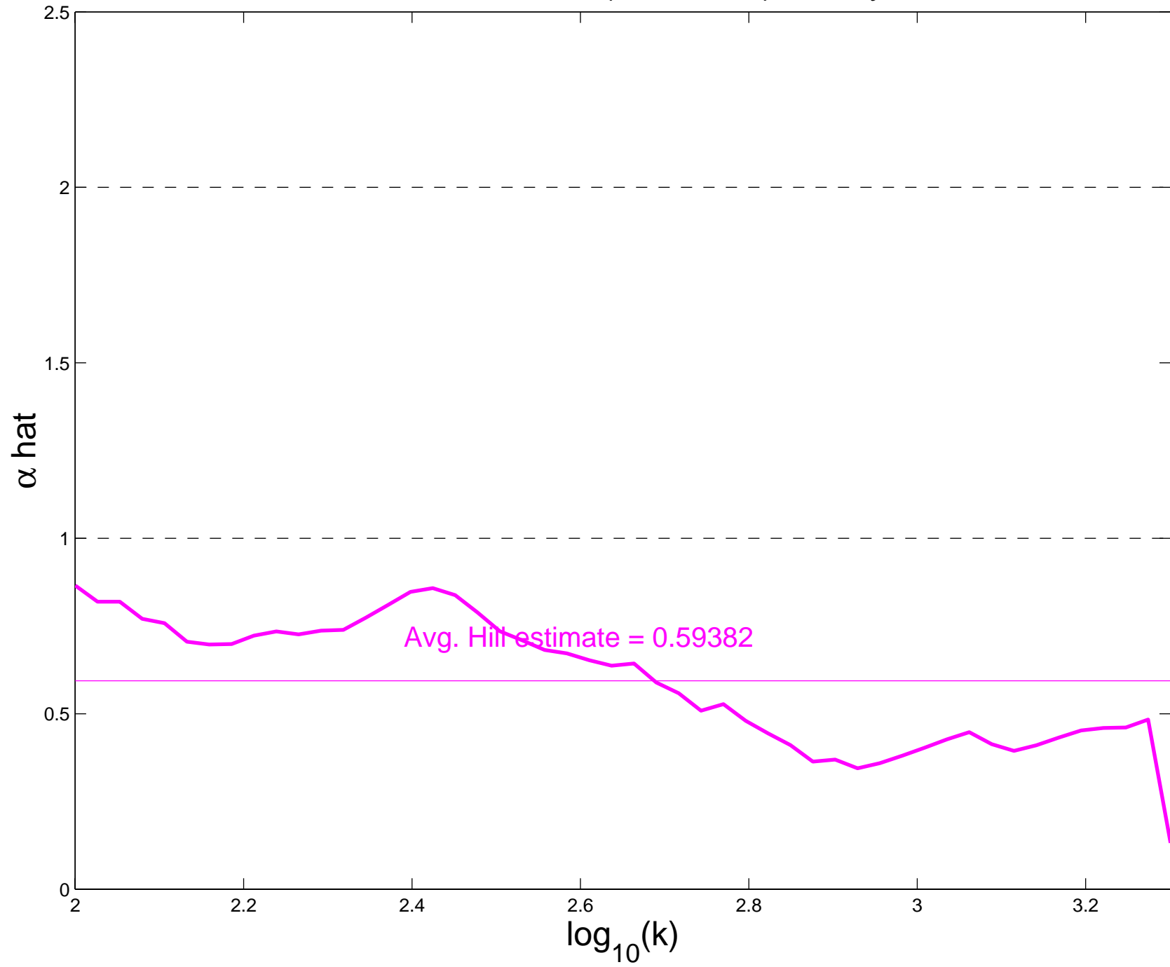
Hill estimates, HTTP Ratio (Size/Time), Friday, Afternoon
