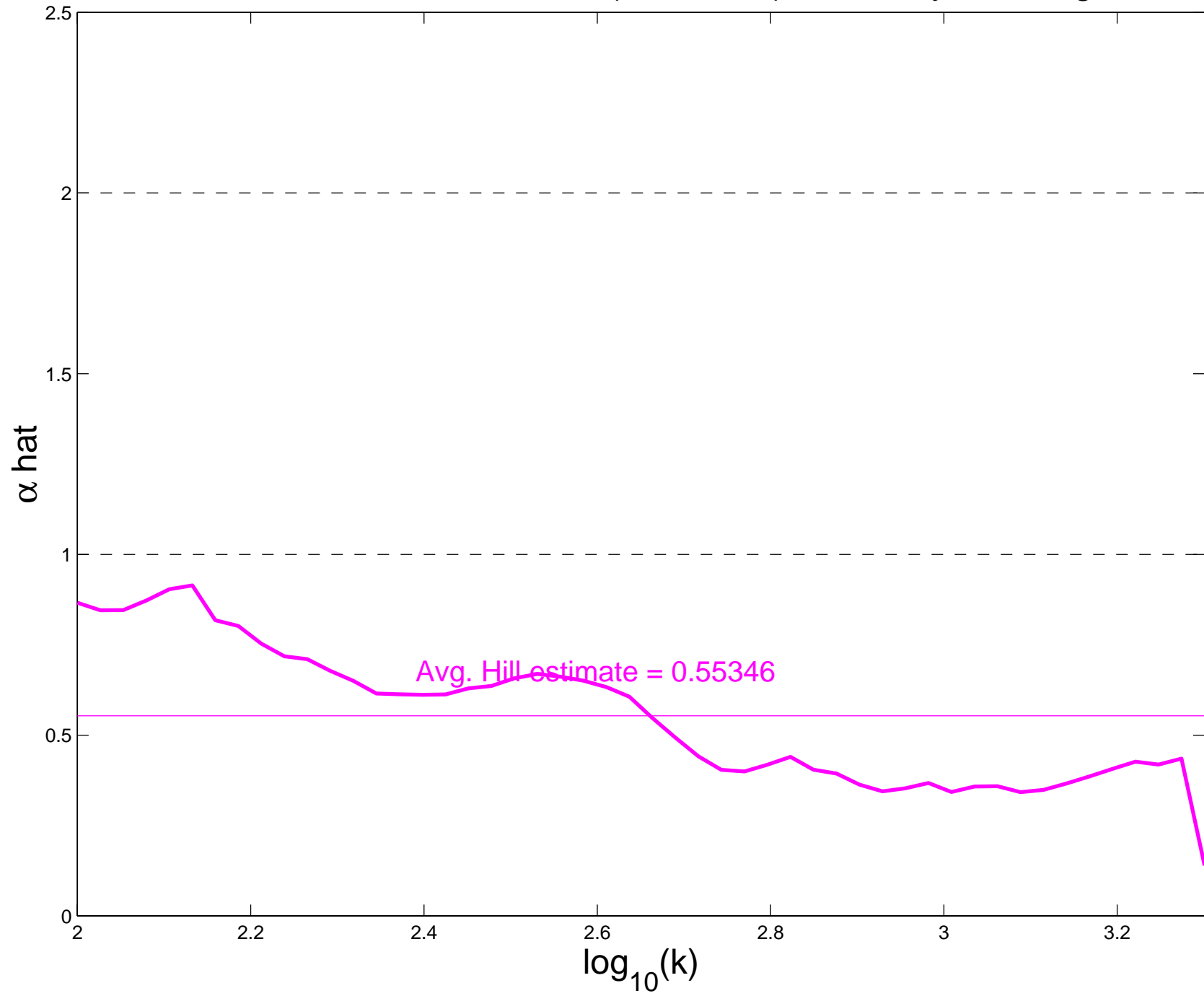
Hill estimates, HTTP Ratio (Size/Time), Thursday, Morning
