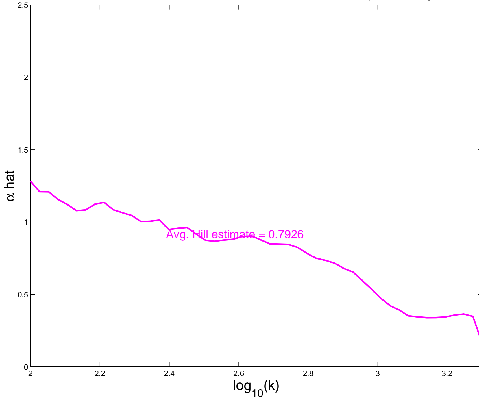
Hill estimates, HTTP Ratio (Size/Time), Monday, Morning
