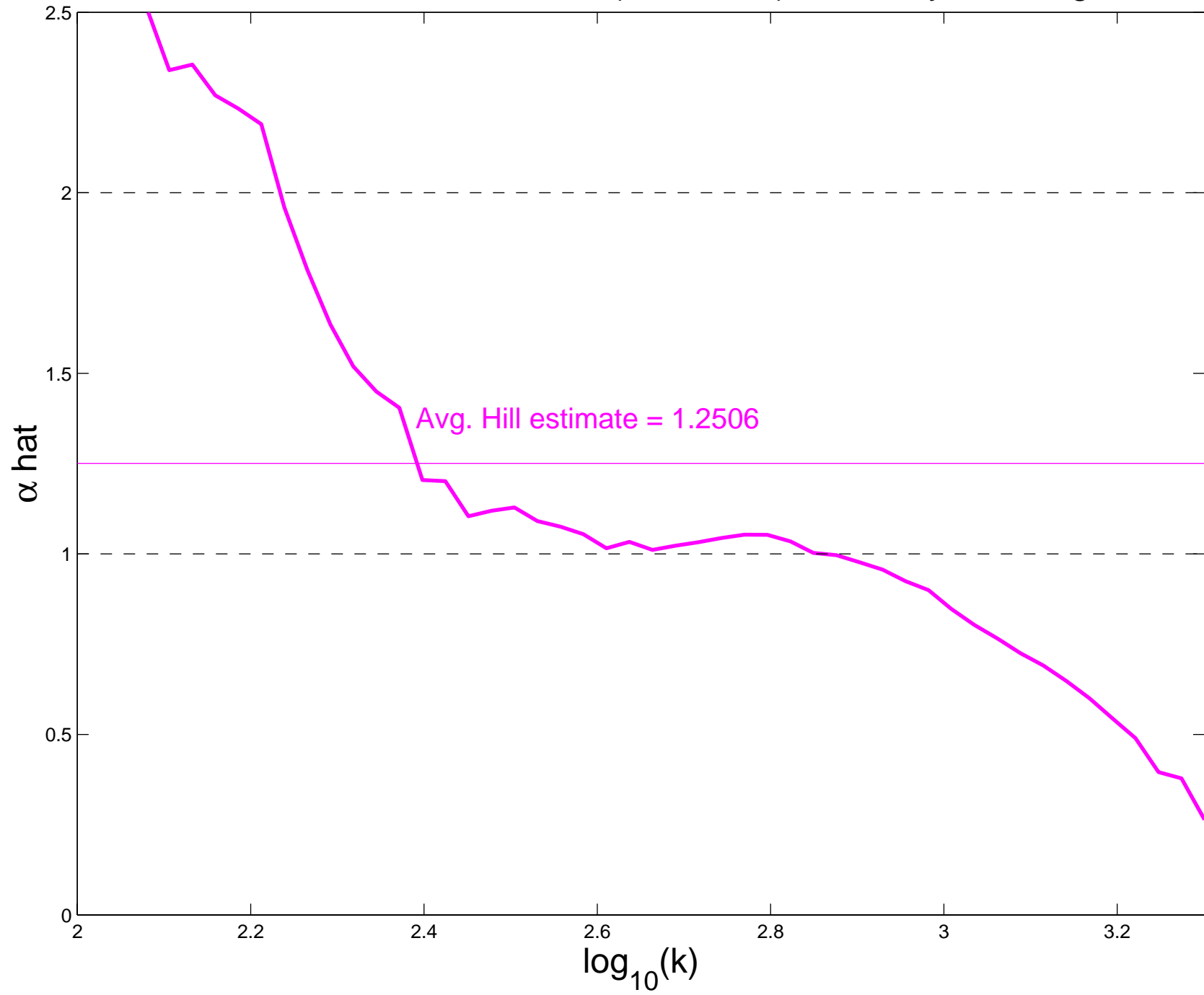
Hill estimates, HTTP Ratio (Size/Time), Saturday, Morning
