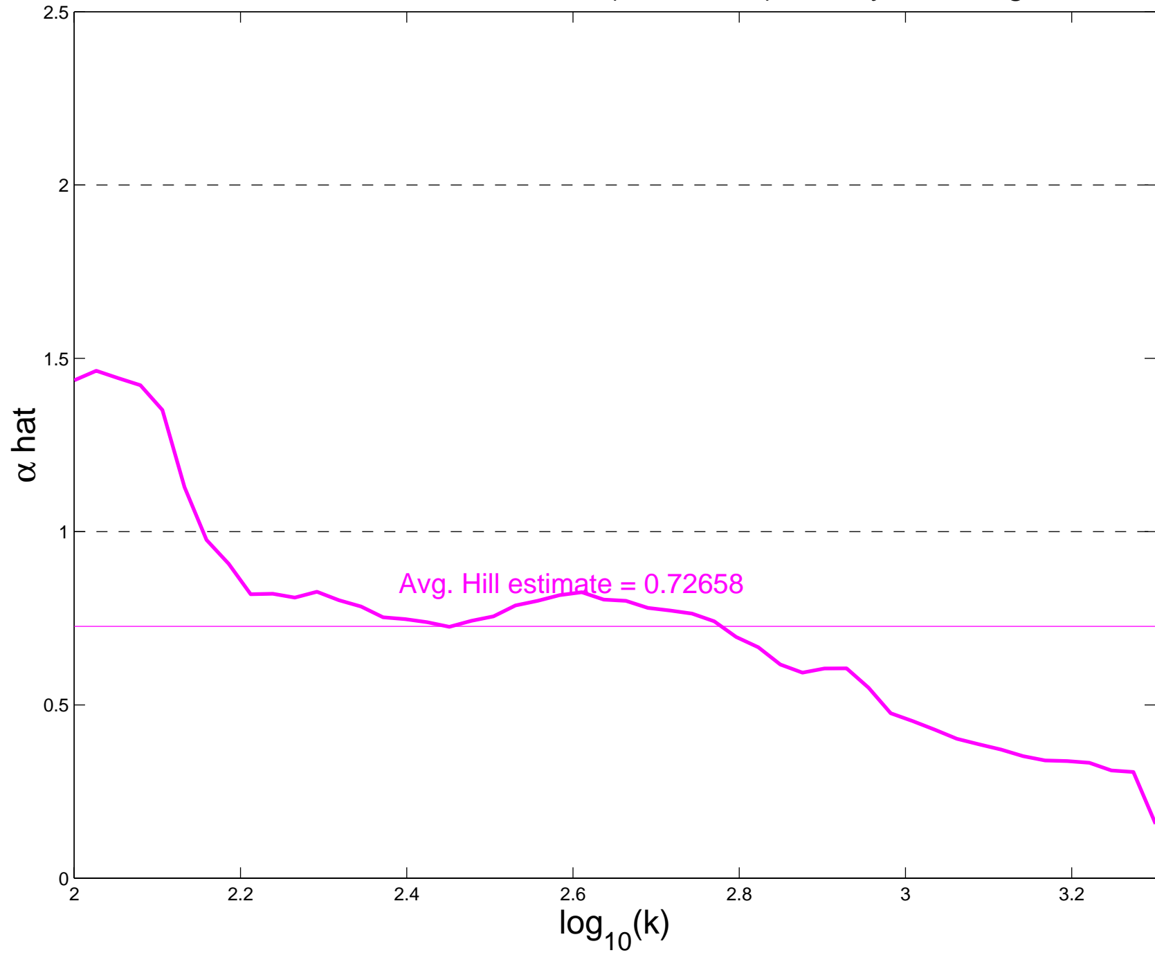
Hill estimates, HTTP Ratio (Size/Time), Friday, Evening
