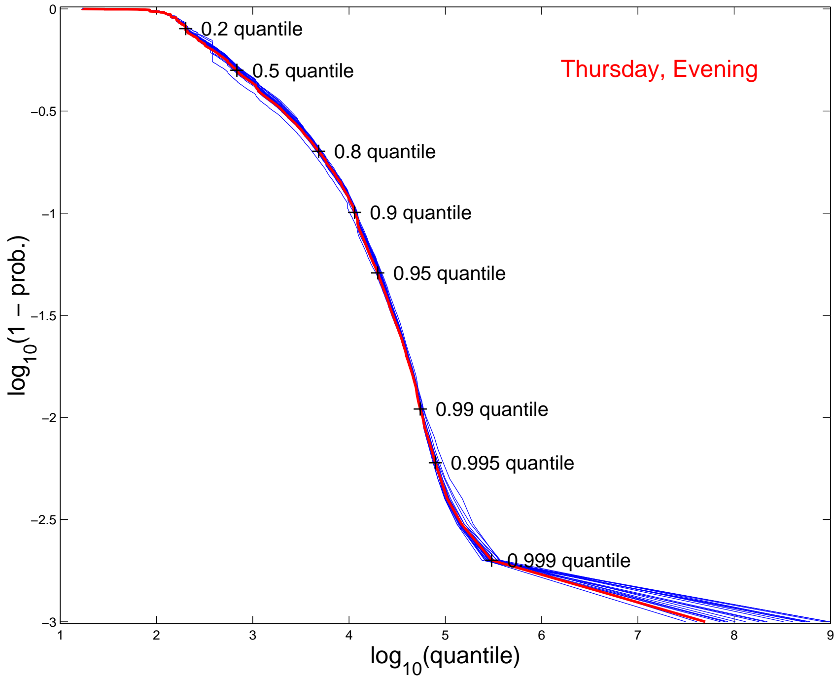
log-log CCDF, HTTP R. S., n = 3034391
