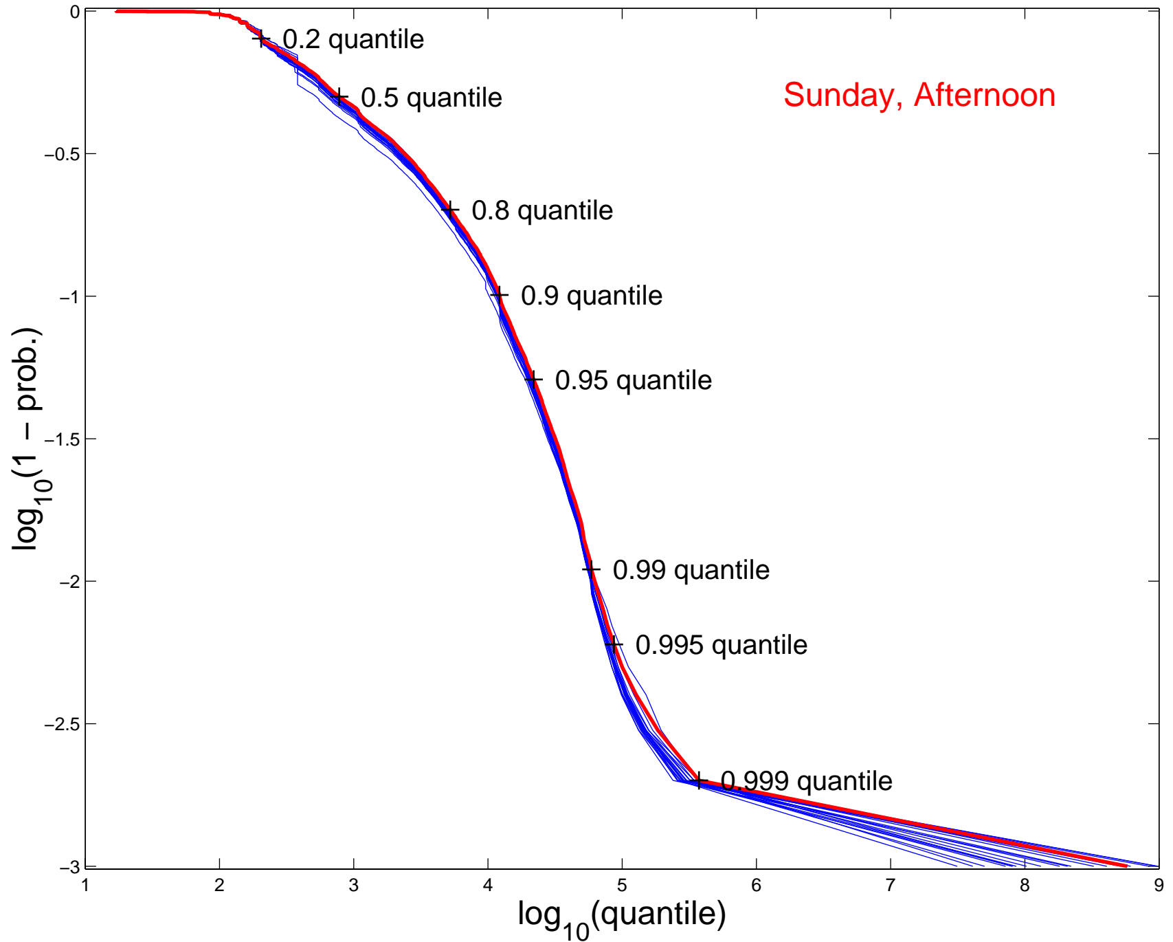
log-log CCDF, HTTP R. S., n = 2973175
