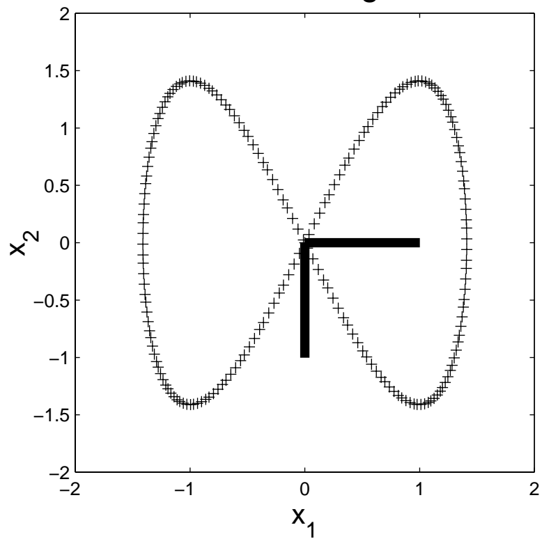
Sin & Sin 2, ICA eigenvectors
