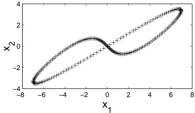
Sin & Sin 2, Mixed Signal Scatterplot
