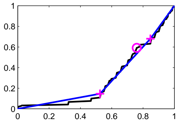
3 knot PW linear fit
